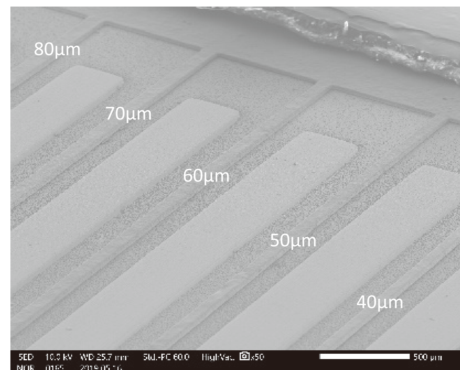
40μm~80μm Solder Dam (Copper Thickness 35μm)
