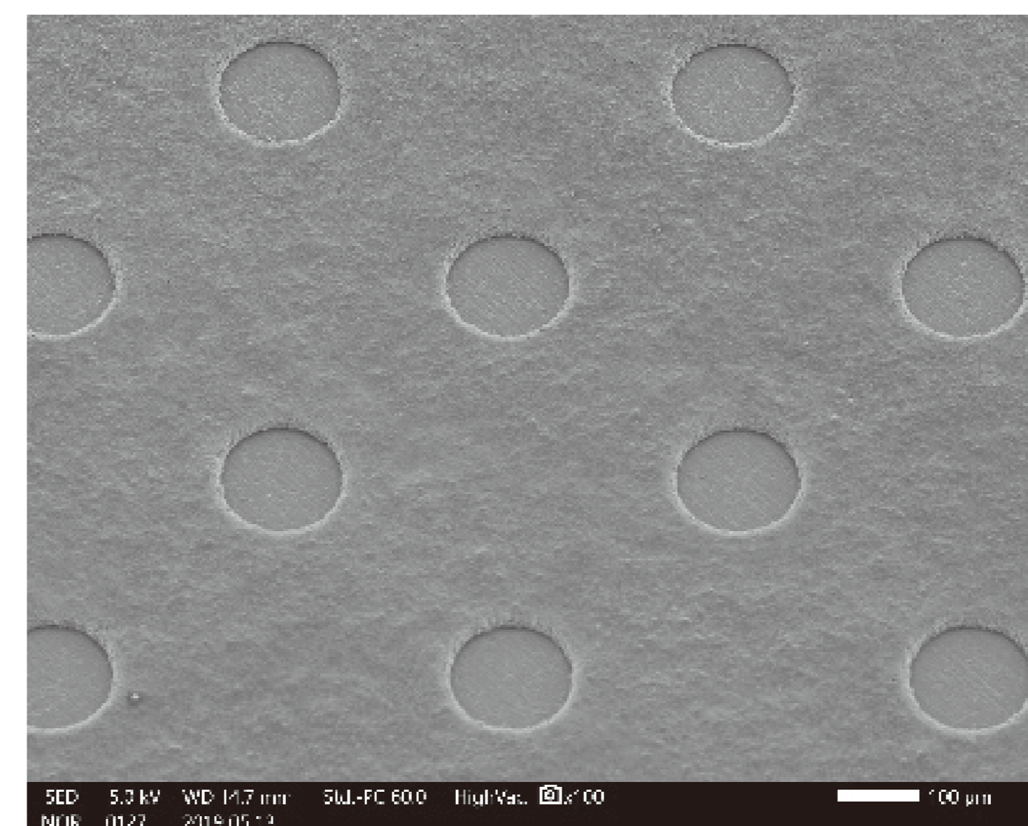
200μm Via on copper
