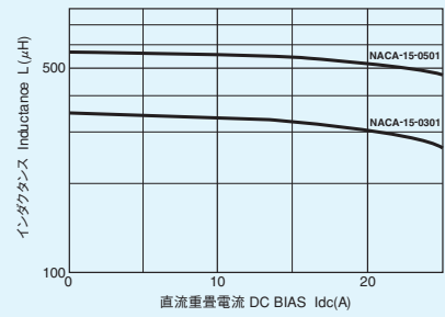
NACA-15 Series
